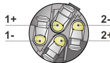
Speakon NL4FC
