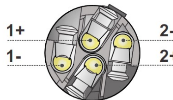
Speakon NL4FC
